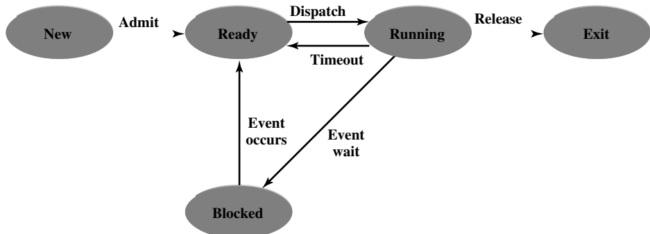
Figure 8.7 Five-State Process Model
