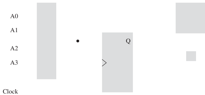
Figure 20.35 A Simple FPGA Logic Block
