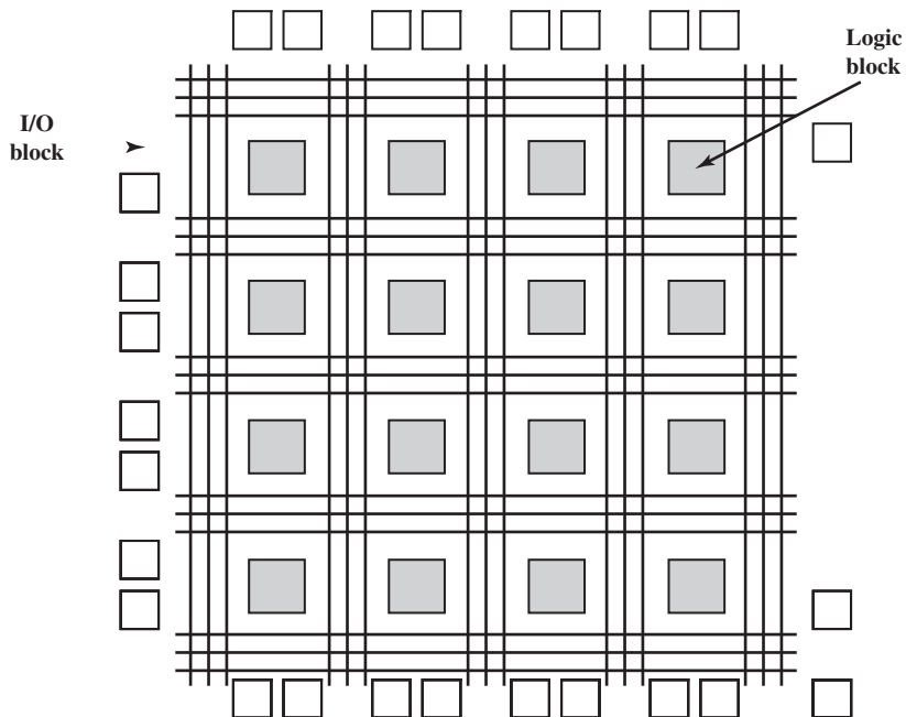
Figure 20.34 Structure of an FPGA
