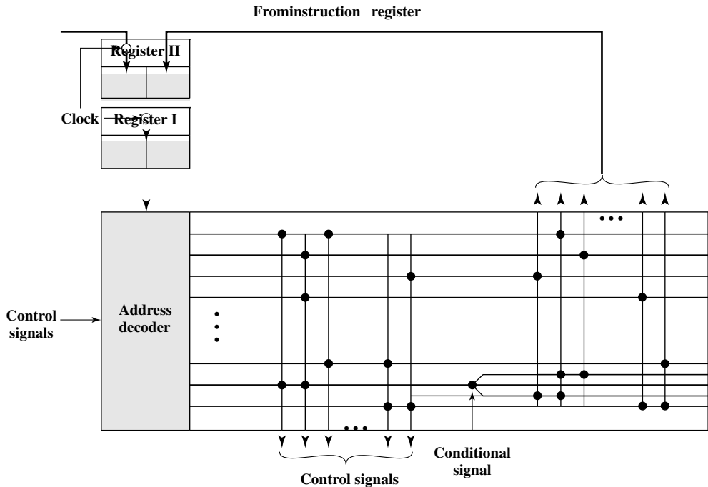
Figure 16.5 Wilkes's Microprogrammed Control Unit
