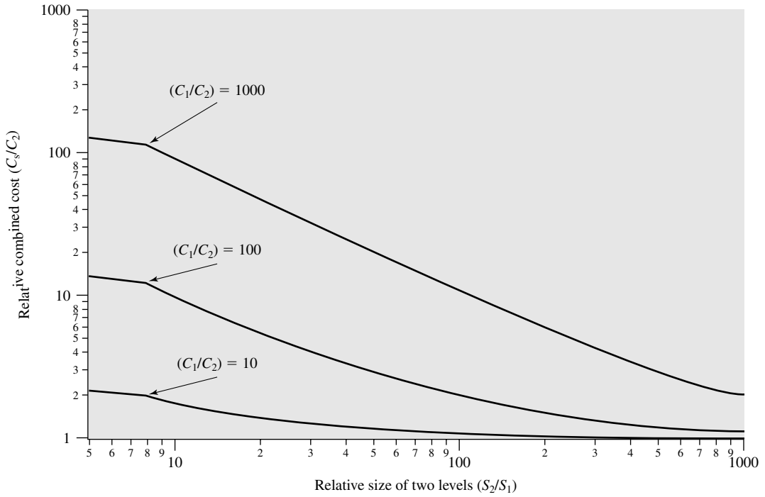
Figure 4.22 Relationship of Average Memory Cost to Relative Memory Size for a Two-Level Memory
