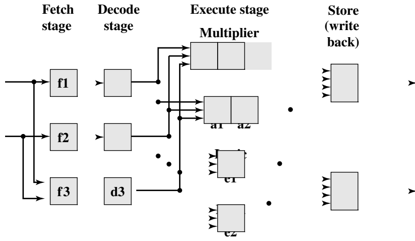
Lookahead window Figure 14.14 A Dual-Pipeline Superscalar Processor
