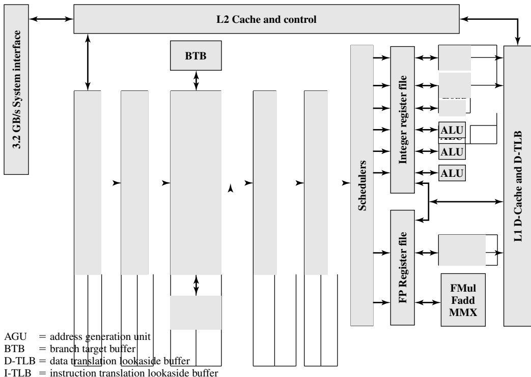
Figure 14.7 Pentium 4 Block Diagram
