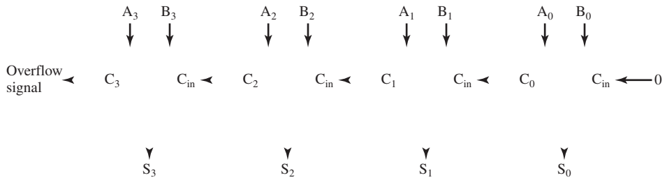
Figure 20.19 4-Bit Adder
