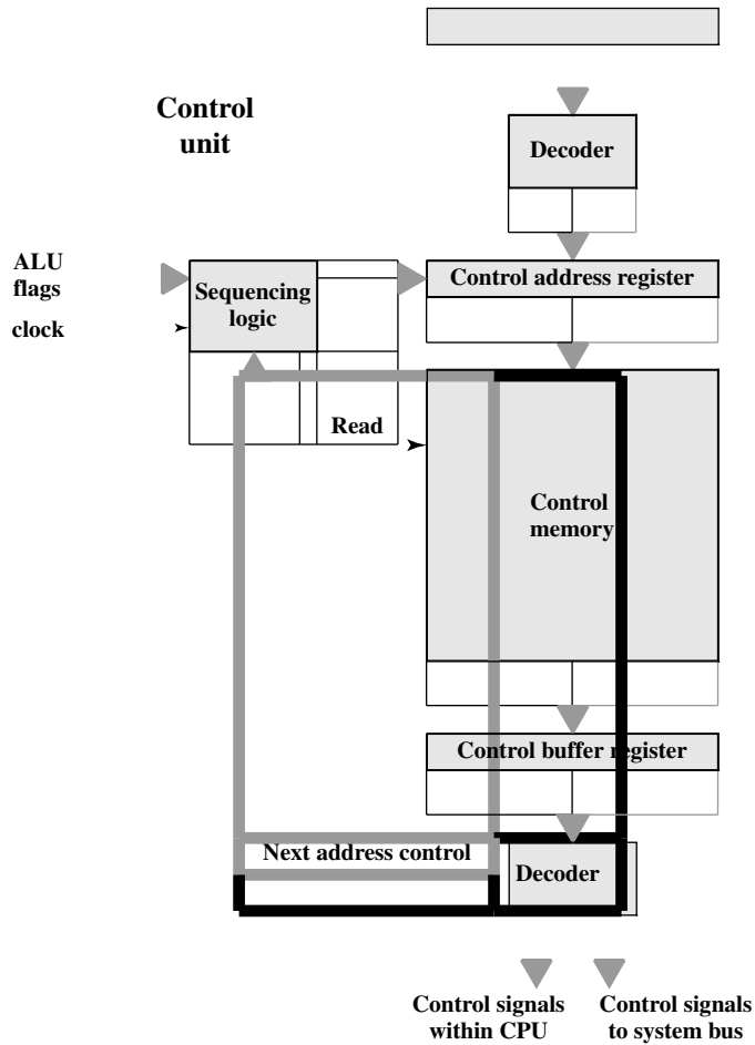
Figure 16.4 Functioning of Microprogrammed Control Unit
