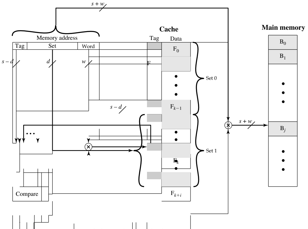
Figure 4.14 K-Way Set Associative Cache Organization
