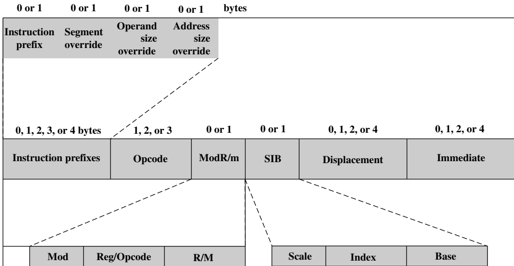
Figure 11.9 x86 Instruction Format
