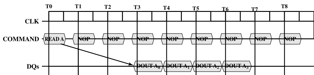
Figure 5.13 SDRAM Read Timing (burst length = 4)
