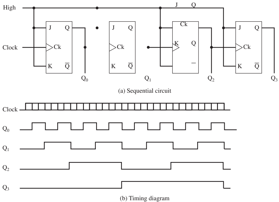
Figure 20.30 Ripple Counter
