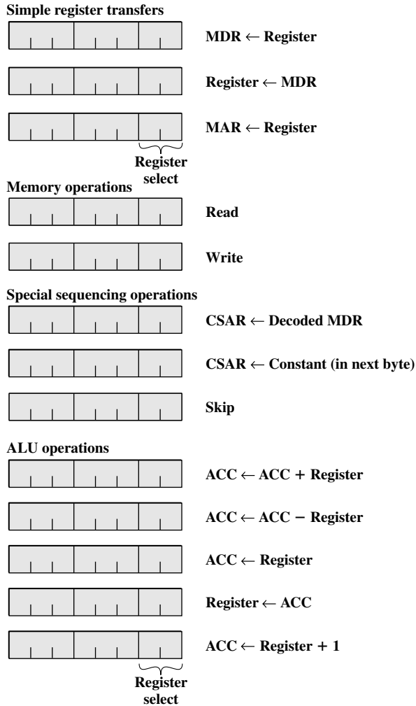
(a) Vertical microinstruction format
