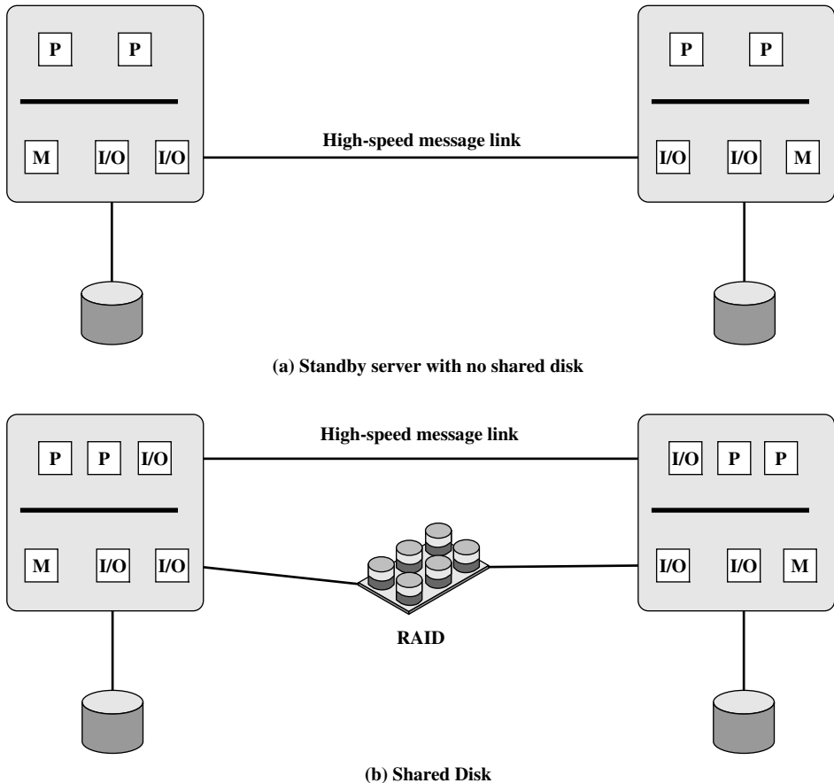
Figure 17.10 Cluster Configurations
