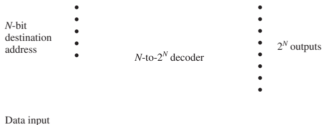
Figure 20.17 Implementation of a Demultiplexer Using a Decoder
