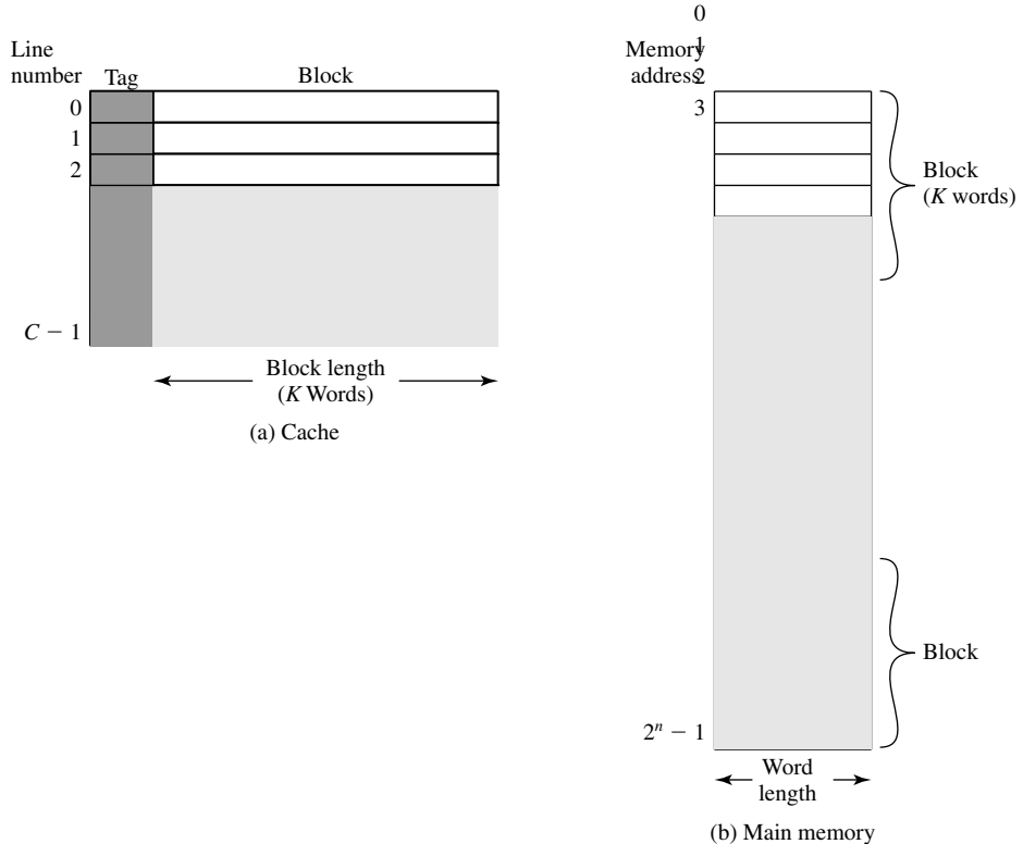
Figure 4.4 Cache/Main Memory Structure
