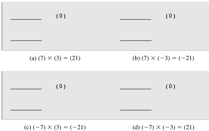
Figure 9.14 Examples Using Booth's Algorithm
