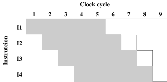
(a) Five-stage pipeline, ideal case
