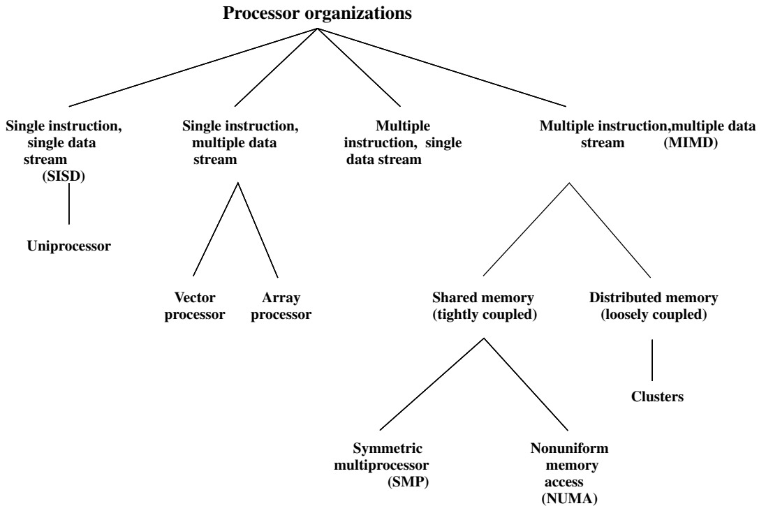
Figure 17.1 A Taxonomy of Parallel Processor Architectures
