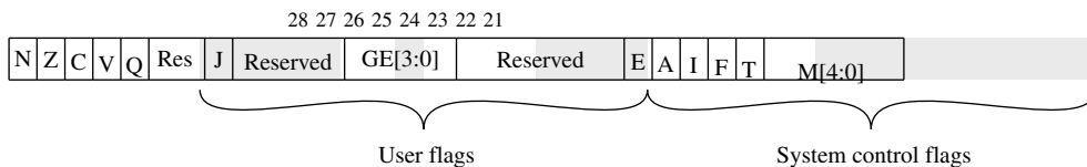
Figure 12.27 Format of ARM CPSR and SPSR
