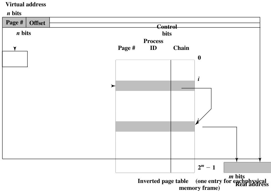
Figure 8.17 Inverted Page Table Structure
