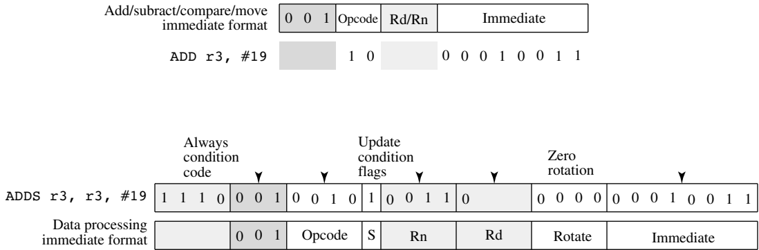
Figure 11.12 Expanding a Thumb ADD Instruction into its ARM Equivalent
