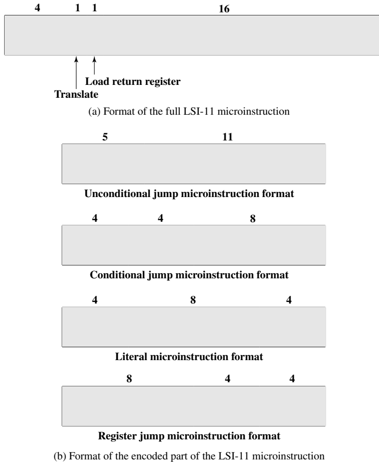
Figure 16.15 LSI-11 Microinstruction Format
