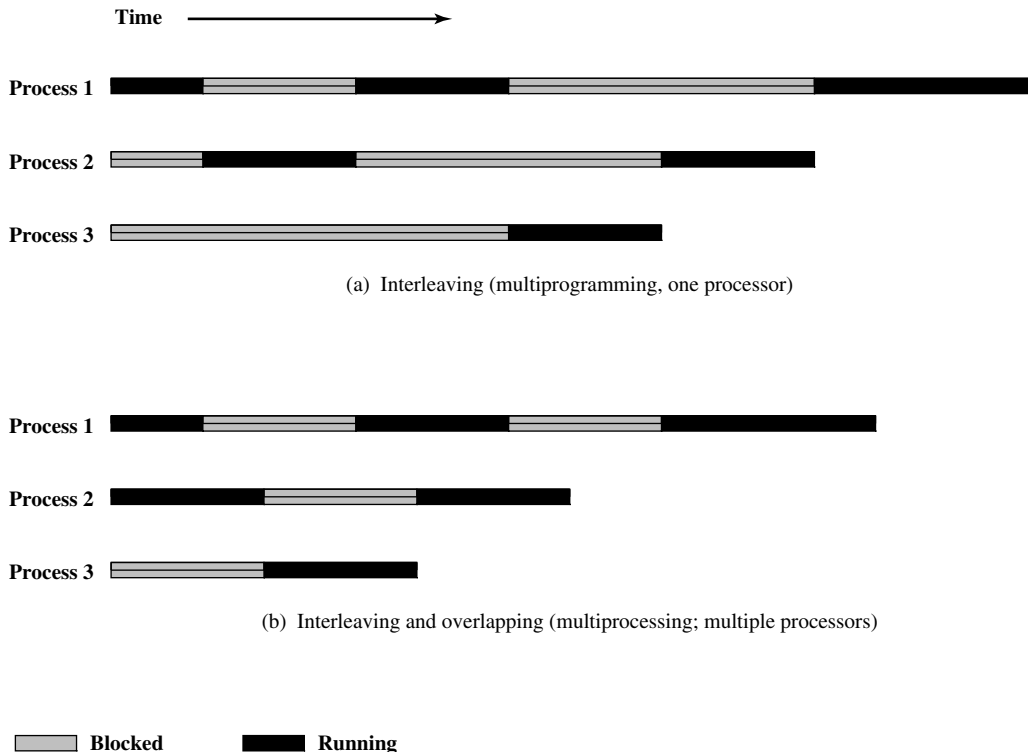
Figure 17.3 Multiprogramming and Multiprocessing
