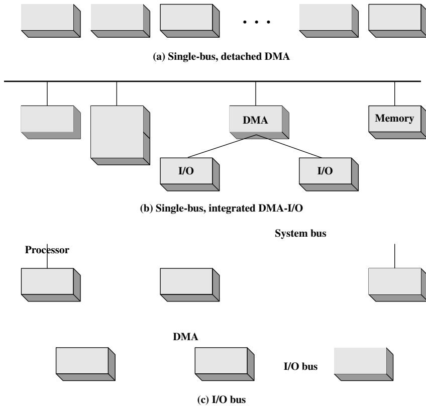
Figure 7.13 Alternative DMA Configurations
