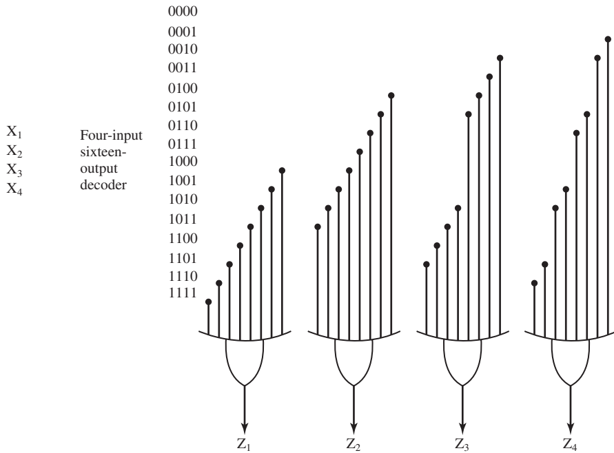
Figure 20.18 A 64-Bit ROM
