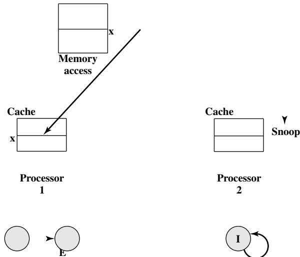
Figure 17.22 MESI Example: Processor 1 Reads Line x
