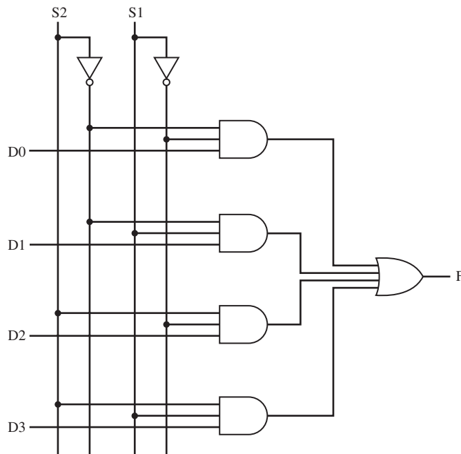
Figure 20.13 Multiplexer Implementation
