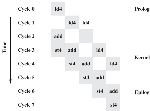
Figure 21.6 Software Pipelining Example
