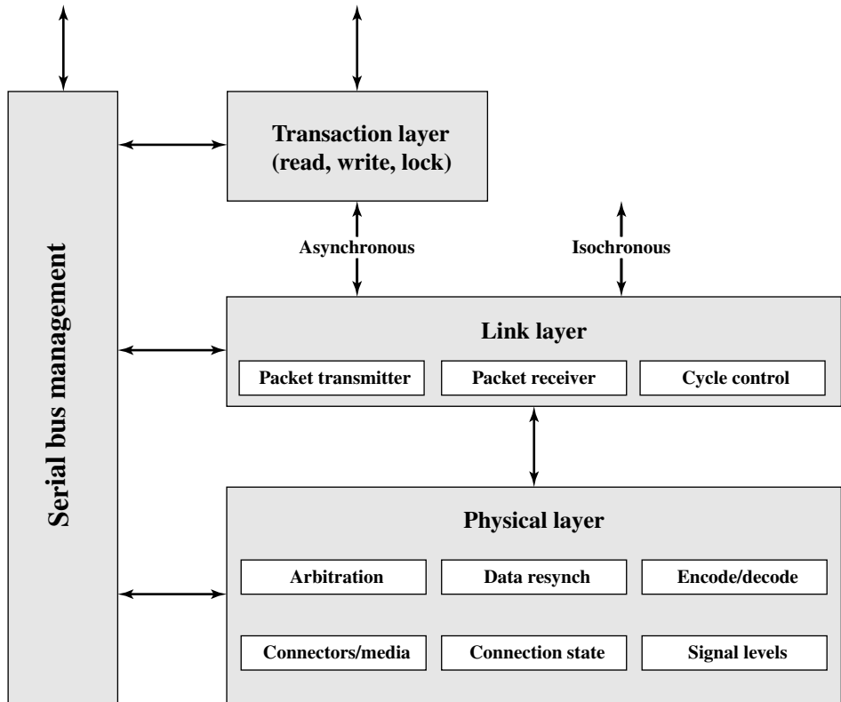
Figure 7.18 FireWire Protocol Stack
