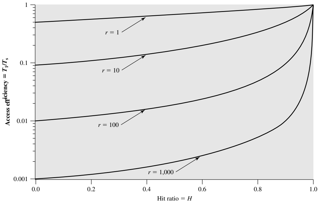
Figure 4.23 Access Efficiency as a Function of Hit Ratio ( r =
