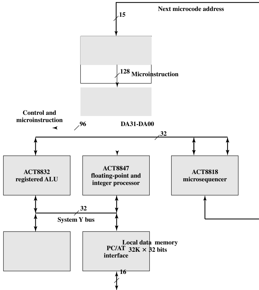
TI 8800 Block Diagram
