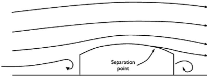
Figure 10.2 Flow separations over arched roofs (from Blessmann, 1991).
