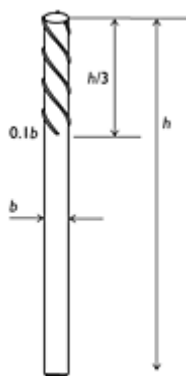
Figure 4.23 Helical strakes for inhibiting vortex shedding.
