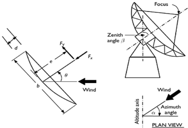
Figure 14.13 Resultant aerodynamic forces on the dish antenna of a radio telescope (Wyatt, 1964).
