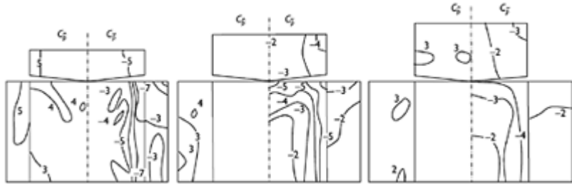
Figure 8.13 Largest maximum and minimum pressure coefficients, \bar{c}_p and \bar{c}_{p, \min} , for industrial buildings with roofs of 5° pitch (for any wind direction) (Davenport et al. , 1977).
