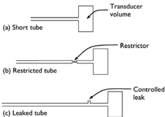
Figure 7.7 Tubing arrangements for measurement of point pressures.
