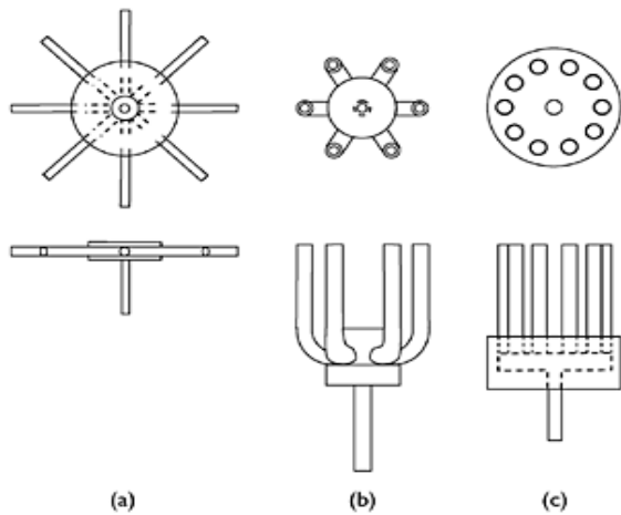
Figure 7.8 Manifolds for pressure averaging.
