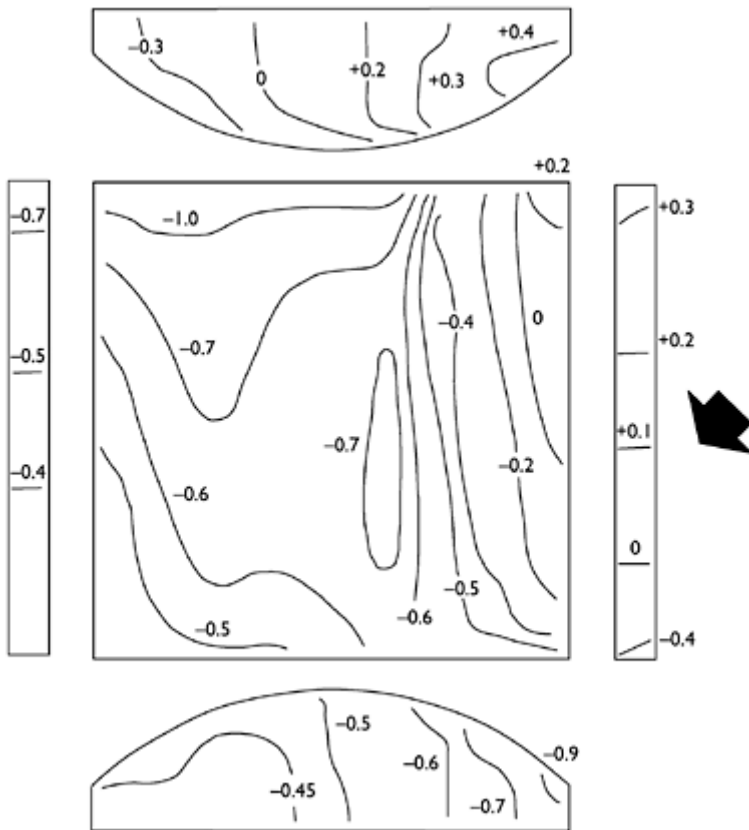
Figure 10.6 Mean pressure coefficients on an arched-roof building—45° (rise/span=0.2).
