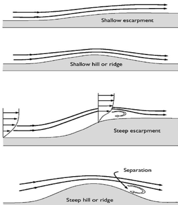
Figure 3.10 Flow over shallow and steep topography.
