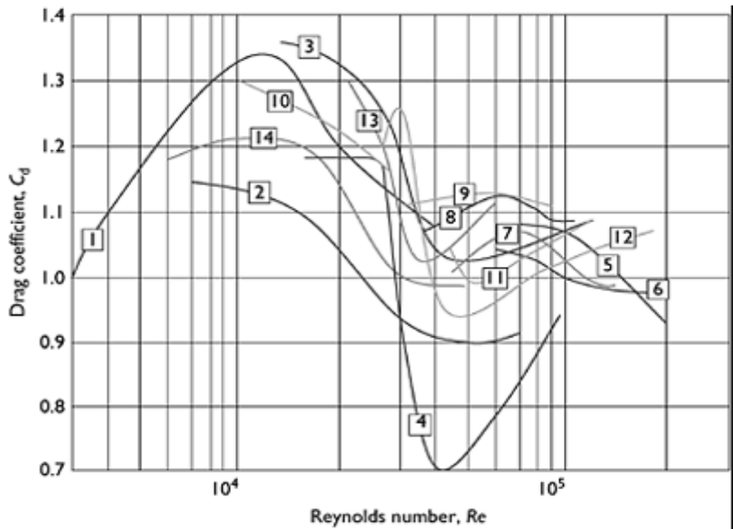
Figure 13.2 Drag force coefficients on conductors from wind-tunnel tests (ASCE, 1990).
