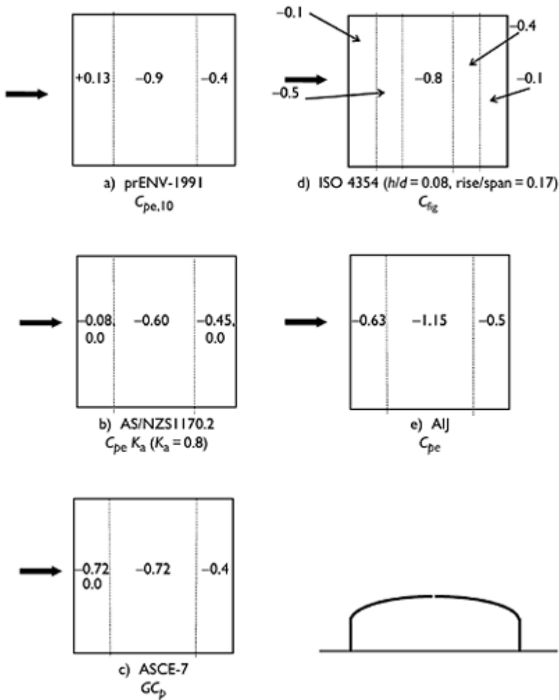
Figure 15.5 Comparison of pressure coefficients for an arched roof (main structural loads), h/d=0.2 , rise/span=0.2 .
