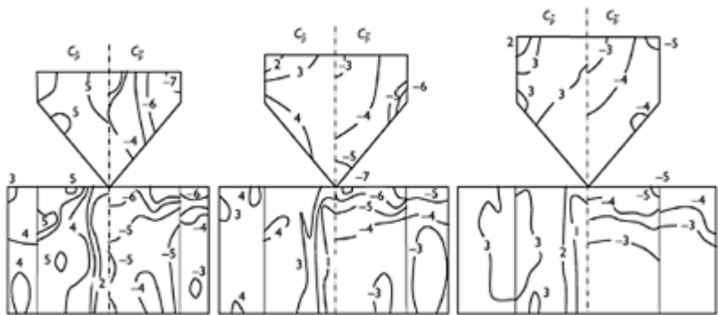
Figure 8.15 Largest maximum and minimum pressure coefficients, \hat{C}_p and \hat{C}_{p,r} for industrial buildings with roofs of 45° pitch (for any wind direction) (Davenport et al. , 1977).
