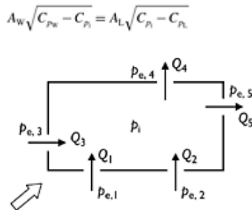
Figure 6.3 Inflows and outflows for multiple openings.
