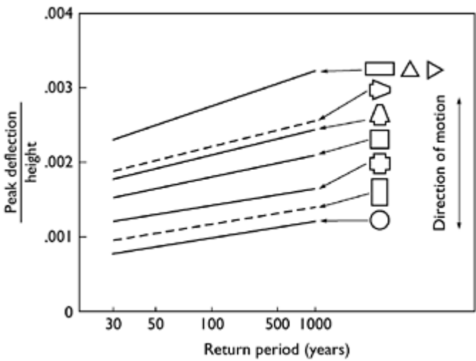
Figure 9.9 Effect of cross-sectional shape on maximum deflections of six buildings (from Davenport, 1971).
