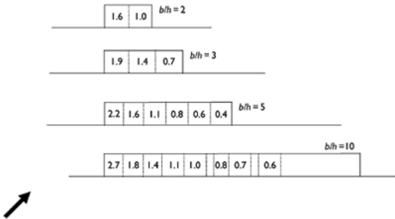
Figure 14.3 Mean pressure difference coefficients for free-standing walls (oblique wind).
