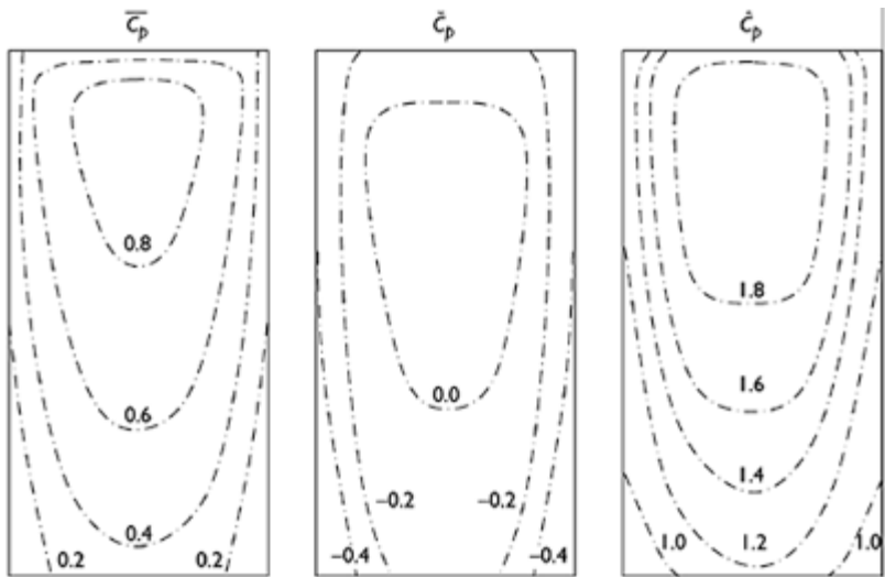
Figure 9.3 Mean, maximum and minimum pressure coefficients—windward wall of a building with square cross-section—height/width=2.1.
