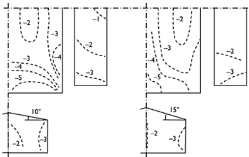
Figure 8.11 Largest minimum pressure coefficients, \bar{C}_{p,r} , for houses with roofs of 10° and 15° pitch (for any wind direction).
