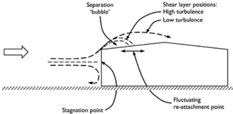
Figure 8.5 Wind flow around a low-rise building.
