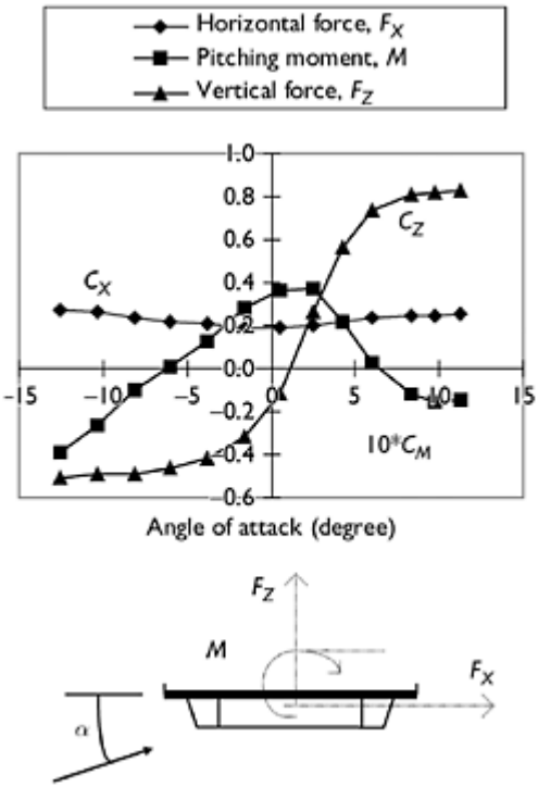
Figure 12.4 Static force coefficients for a typical bridge deck section.
