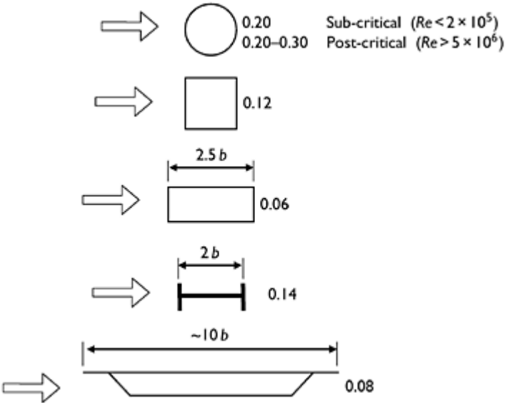
Figure 4.21 Strouhal numbers for vortex shedding for various cross-sections.
