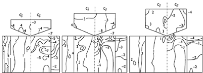
Figure 8.14 Largest maximum and minimum pressure coefficients, \hat{C}_p and \hat{C}_{p,r} for industrial buildings with roofs of 18° pitch (for any wind direction) (Davenport et al. , 1977).
