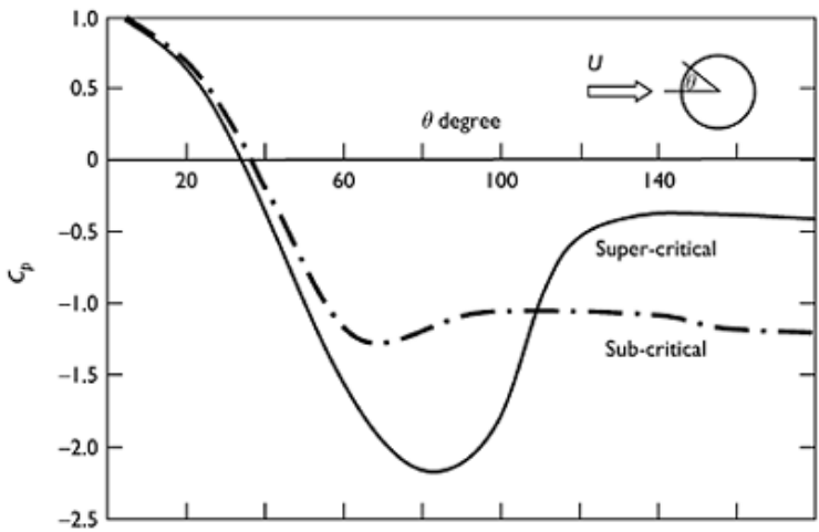
Figure 4.18 Pressure distributions around a two-dimensional circular cylinder at sub-critical and trans-critical Reynolds numbers.
