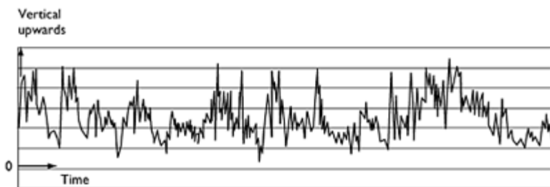
Figure 10.9 Vertical displacement of the leading edge of a cantilevered roof showing some resonant contributions to the response (from Melbourne, 1995).
