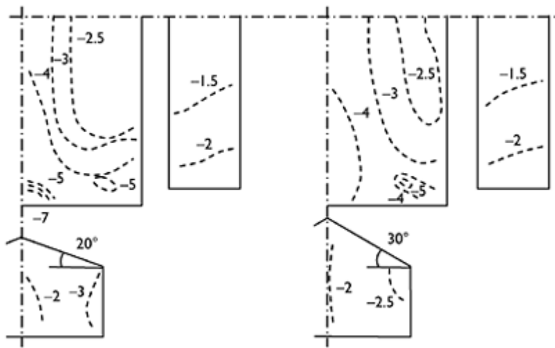
Figure 8.12 Largest minimum pressure coefficients, \bar{c}_{p, \min} , for houses with roofs of 20° and 30° pitch (for any wind direction).
