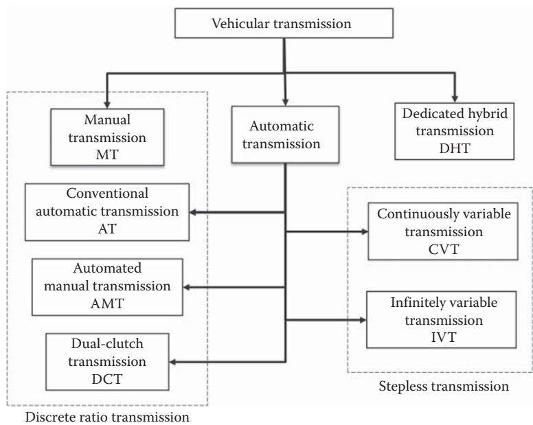
FIGURE 4.7 Classification and types of conventional automotive transmission systems.
