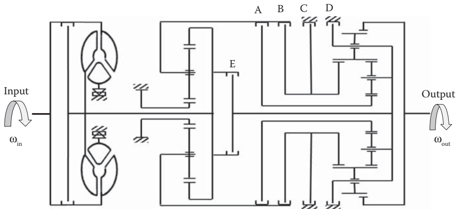
FIGURE 4.22 Lepelletier transmission.
