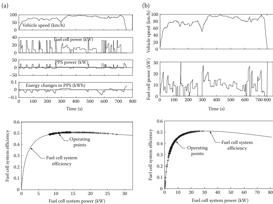
FIGURE 16.9 Operating simulation of fuel cell hybrid and fuel-cell-alone-powered passenger car in FTP75 highway drive cycle: (a) hybrid drivetrain and (b) fuel-cell-alone-powered drivetrain.
