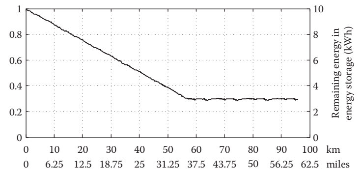
FIGURE 11.19 SOC and remaining energy in energy storage versus traveling distance in FTP75 urban drive cycle in CD mode.
