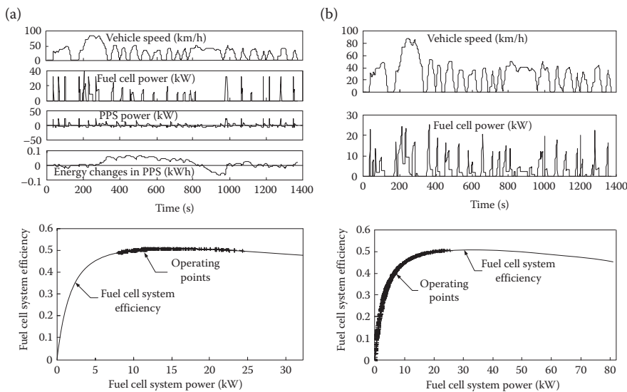
FIGURE 16.8 Operating simulation of fuel cell hybrid and fuel-cell-alone-powered passenger car in FTP75 urban drive cycle: (a) hybrid drivetrain and (b) fuel-cell-alone-powered drivetrain.
