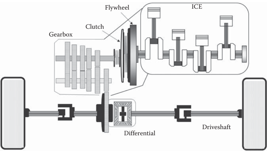
FIGURE 4.8 A typical conventional front wheel powertrain with a manual gearbox.
