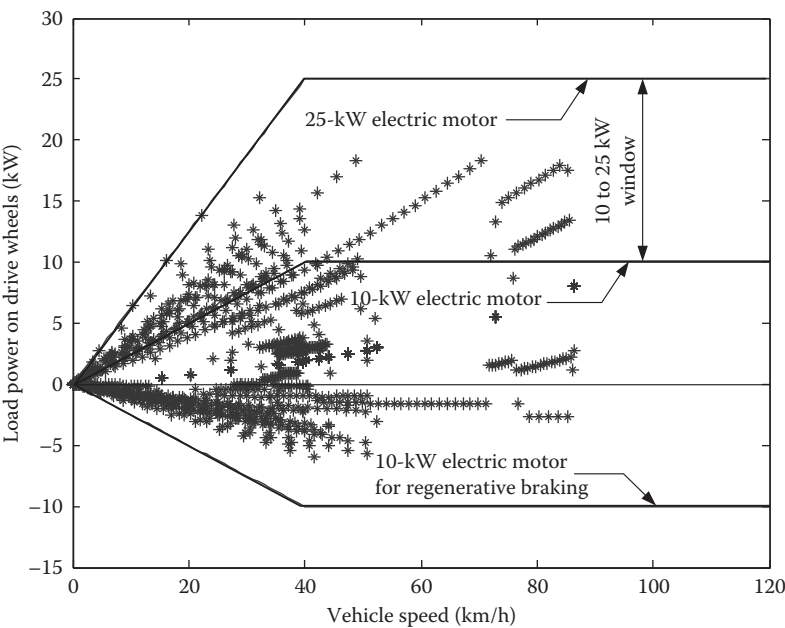
FIGURE 18.10 Load power vs. vehicle speed in FTP75 urban drive cycle for 1200-kg passenger car.
