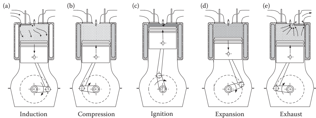
FIGURE 3.2 Four strokes of a SP engine.
